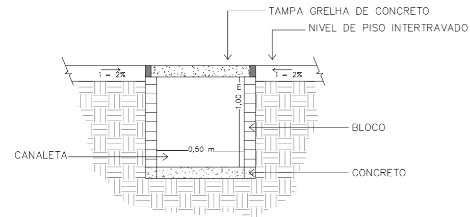
VISTA FRONTAL
