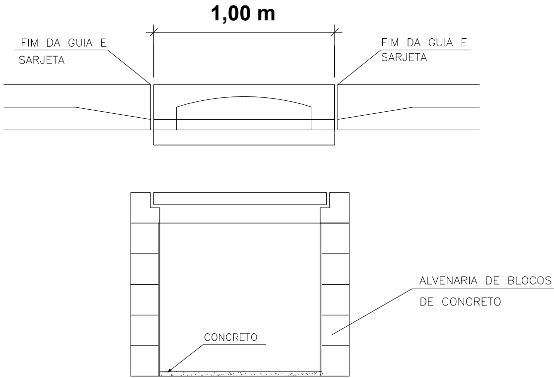
VISTA FRONTAL
